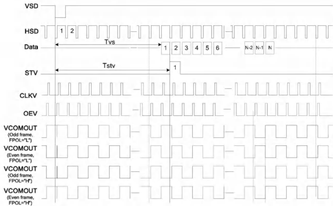
Vertical Timing Diagram (HV Mode)
